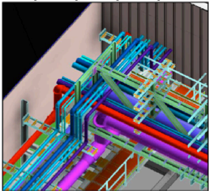
OVERALL MECH ARRANGEMENT
