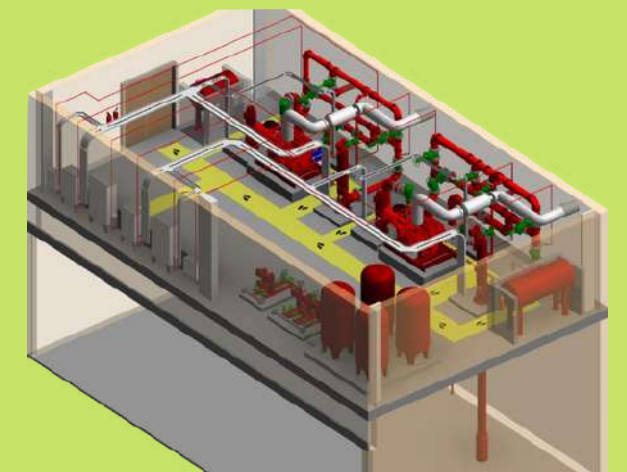
Plumbing & Fire Evacuation Model
