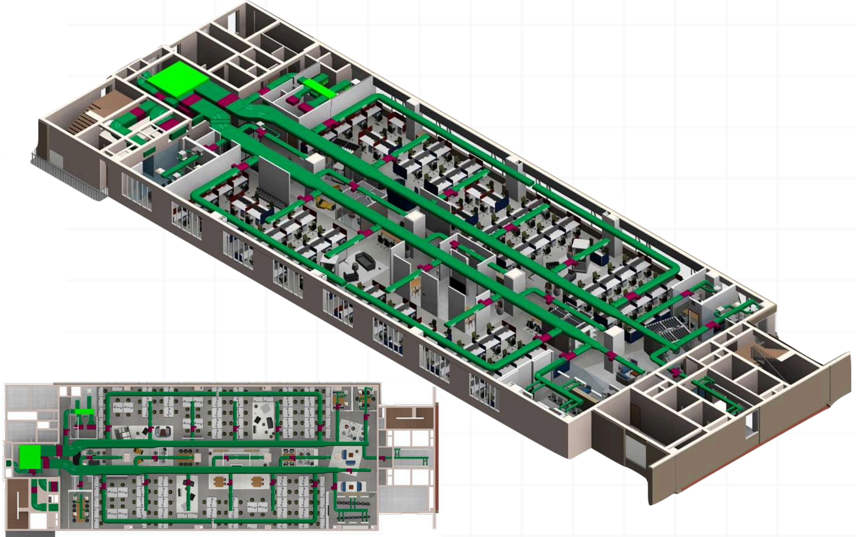
MEP Model - LOD - 300
